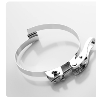
Car-Grip Quick-Fix Clamp Special clamp for attaching Carflex Super and Master-PUR STEP hoses to mobile and stationary installations
